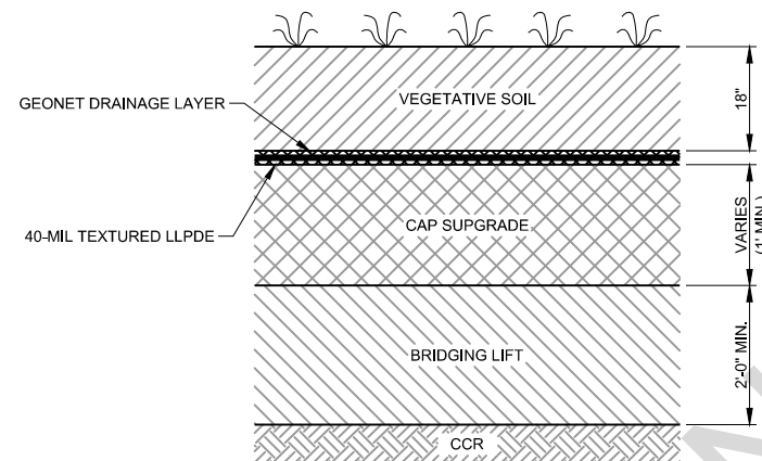
2 7 GEOCOMPOSITE CAP DETAIL NOT TO SCALE
