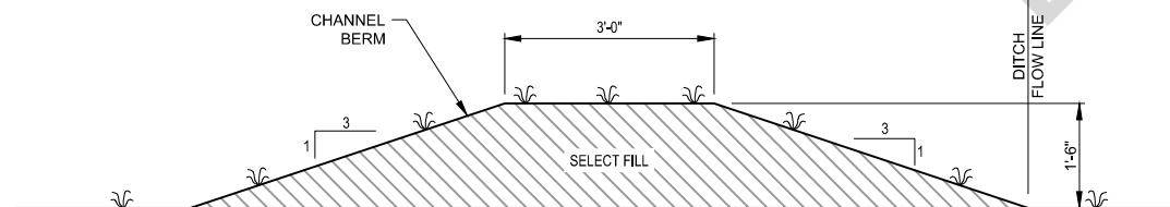
4 7 CHANNEL BERM NOT TO SCALE
