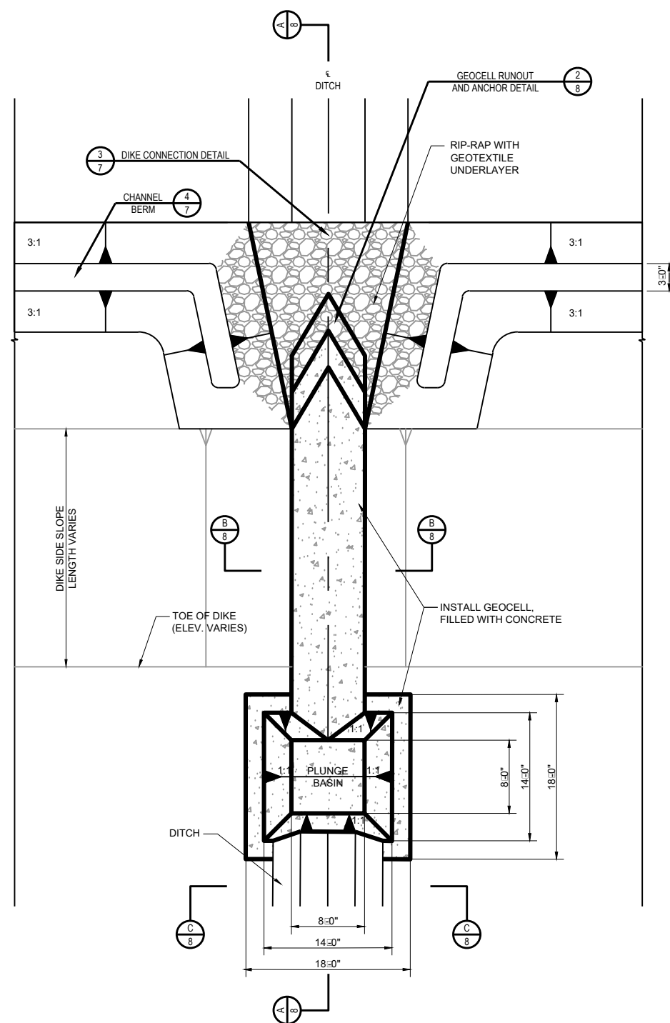
1/8 STORMWATER LET-DOWN STRUCTURE SCALE: 1"=20'
