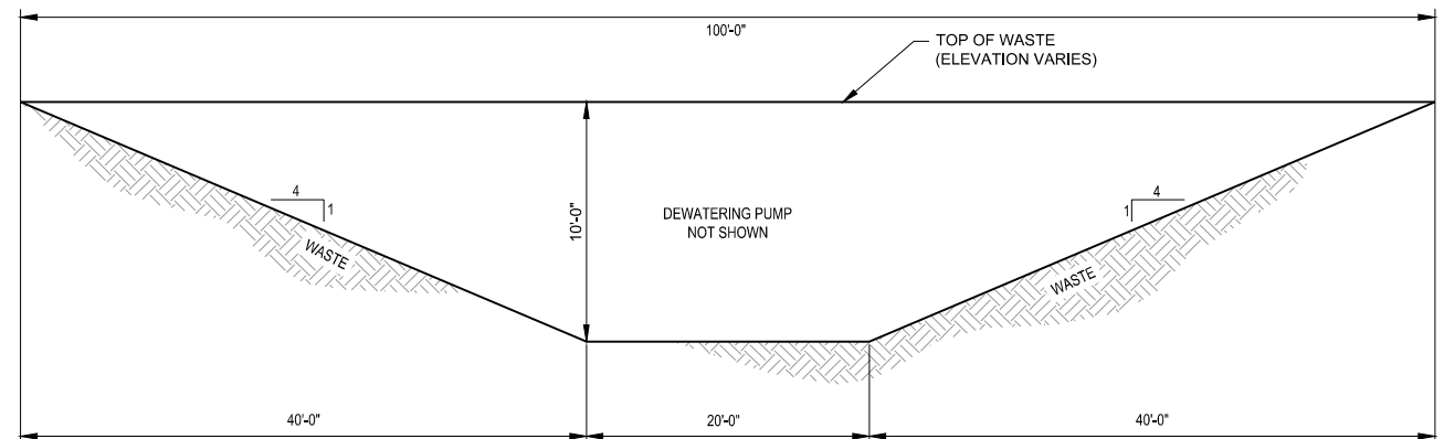
5 7 DEWATERING SUMP DETAIL NOT TO SCALE
